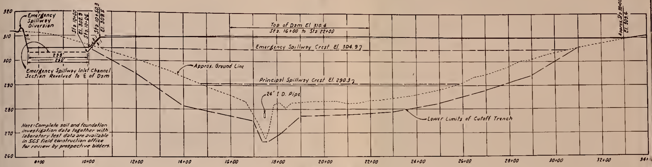
PROFILE ON \mathcal{C} OF DAM
